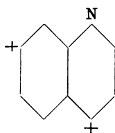
Dahl III.
